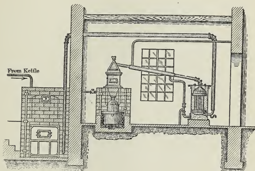
FIG. 16.—Lehmann's Superheated Steam Varnish Apparatus.
